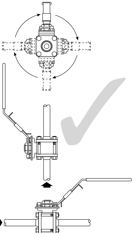
Fig. 4 Correct installation for gas service
